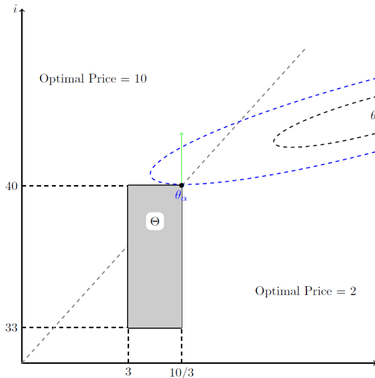
Figure 1: The ellipses are level curves for the KL divergence in the equilibrium of part a where \psi(2) = 35/36 ; the green arrow points in the direction of the greatest KL improvement.
