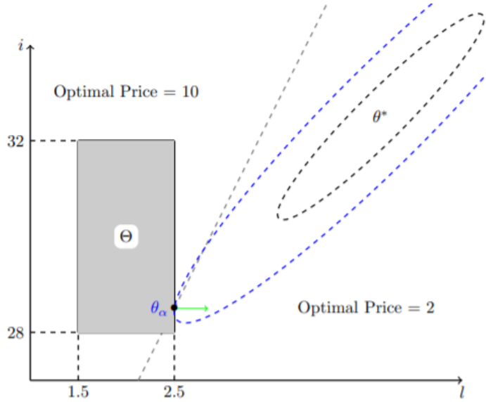
Figure 2: The ellipses are level curves for the KL divergence in the unique equilibrium of part b; the green arrow points in the direction of the greatest KL improvement.
